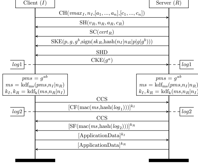
Fig. 3: Message sequence diagram for TLS 1.2 with (EC)DHE key-exchange in unilateral certificate-based server-authentication mode. Optional parameters are omitted.
