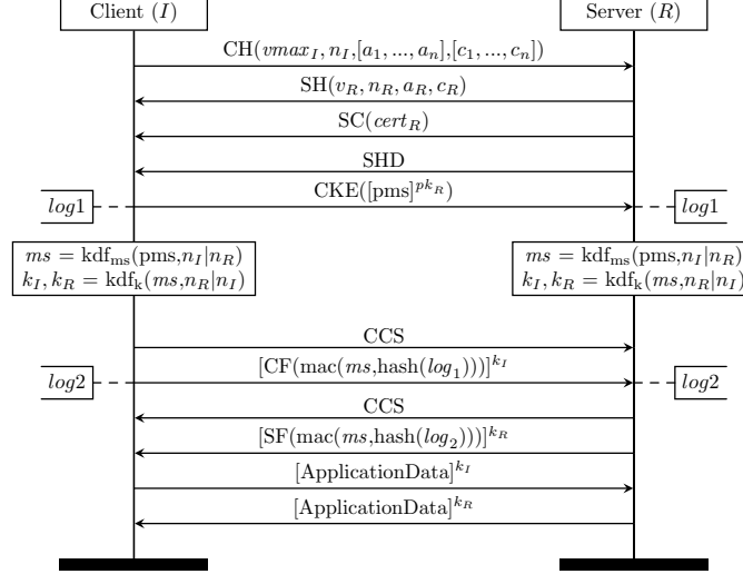
Fig. 4: Message sequence diagram for TLS 1.2 with RSA key-exchange in unilateral certificate-based server-authentication mode. Optional parameters are omitted.
