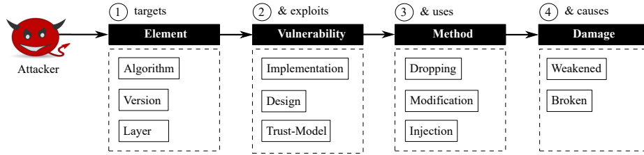
Fig. 2: A taxonomy of downgrade attacks in the TLS protocol and the application protocols using TLS.
